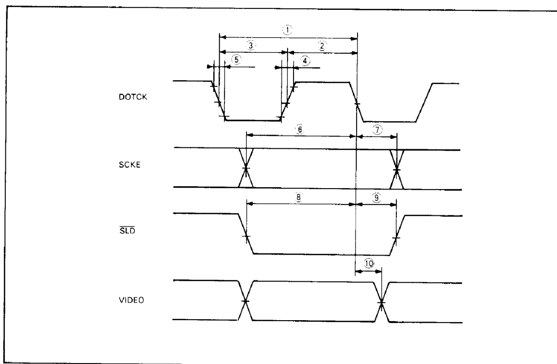
Figure 18. Dot Clock
