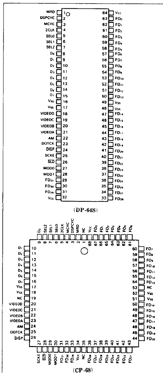
Figure 1. Pin Arrangement
