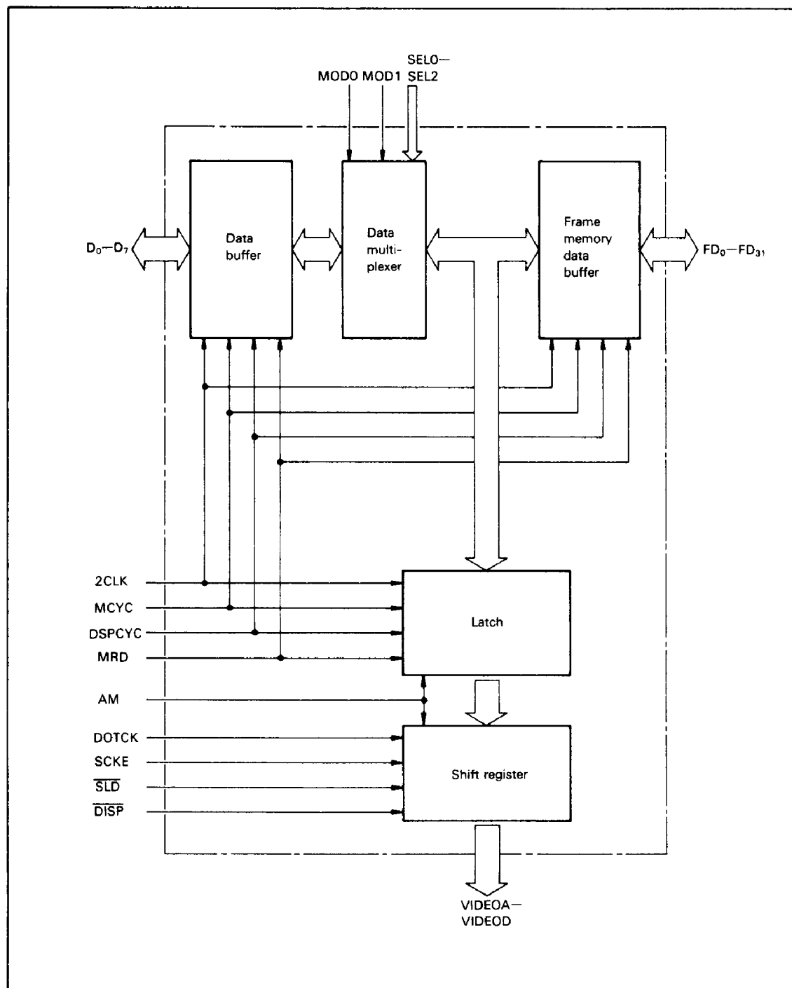
Figure 2. GVAC Block Diagram
